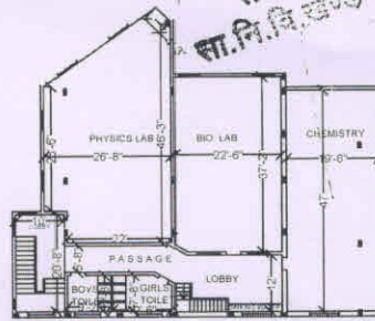
FIRST FLOOR PLAN (BLOCK-B)
