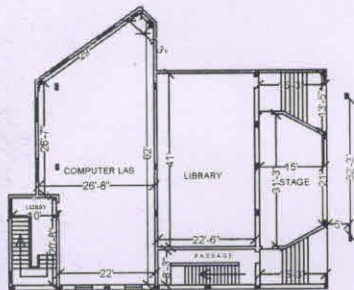
GROUND FLOOR PLAN (BLOCK-B)
