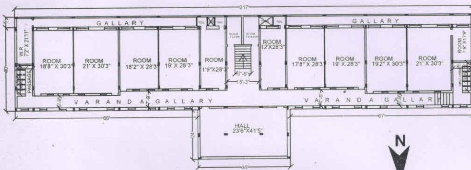
SECOND FLOOR PLAN (BLOCK-A)
