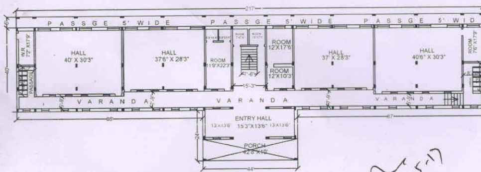
GROUND FLOOR PLAN (BLOCK-A)
