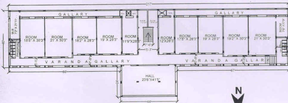
FIRST FLOOR PLAN (BLOCK-A)
